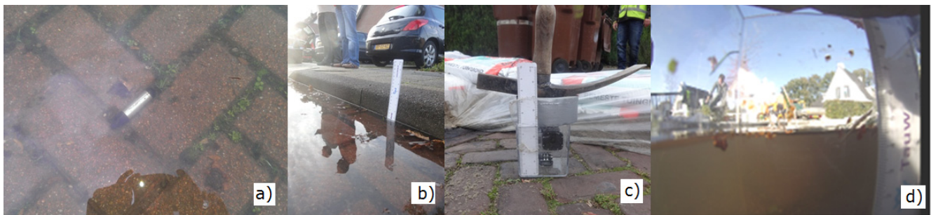
Figure 6. (a) Minidiver installed at lowest point of pavement; (b) hand measurement point; (c) underwater camera set-up; (d) underwater camera view.
